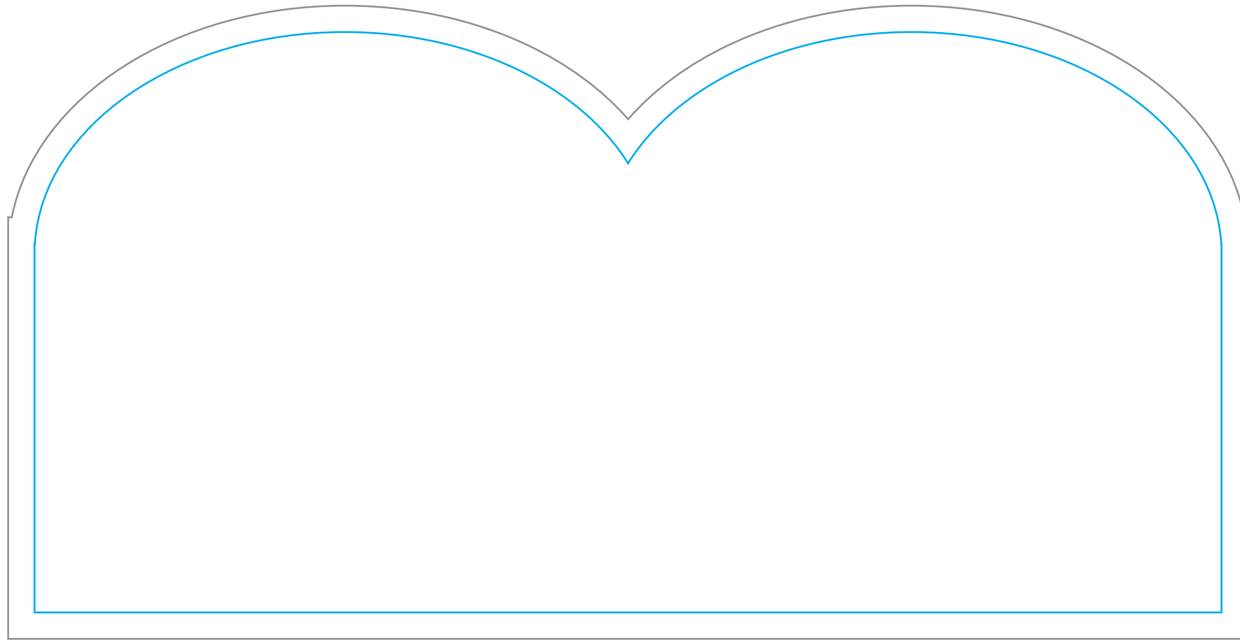
COOLER - 5MM THICKNESS NEOPRENE (TRIM SIZE: 225W x 110Hmm)
